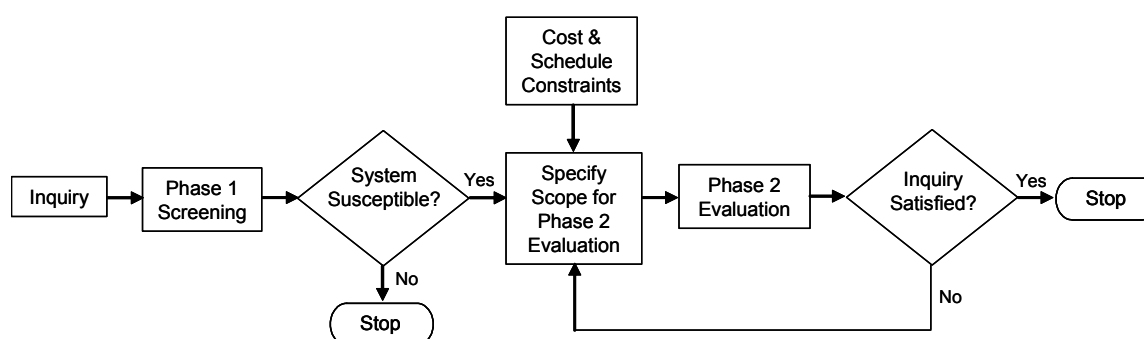
Figure 3-1. Basic Roadmap for System Performance Assessment
