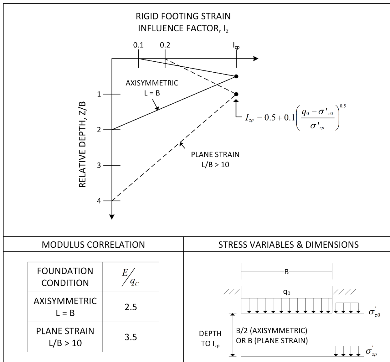
Figure 5-7 Influence Diagram and Modulus Correlation for Schmertmann CPT Method (Schmertmann 1970, Schmertmann et al. 1978)
