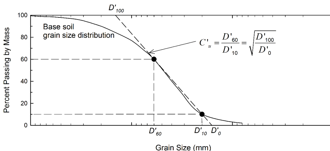
Figure 6-18 Linear Coefficient of Uniformity (after Giroud 2010)
