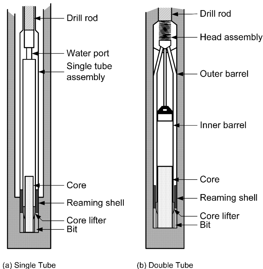
Figure 2-5 Rock Core Samplers (after NCHRP 2018)
