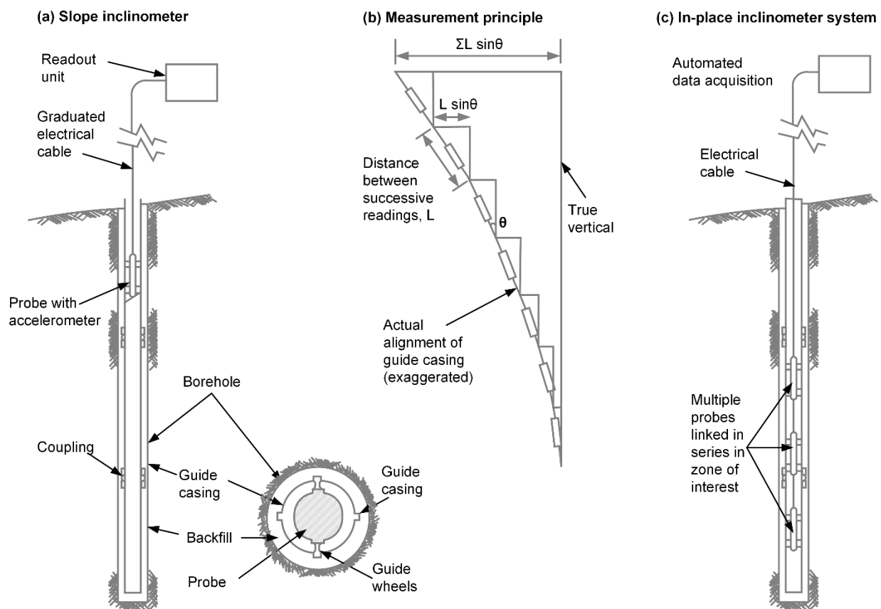
Figure 2-28 Slope Inclinometers – (a) Manual System, (b) Measurement Principle, and (c) In-Place Inclinator System (after Dunnicliff 1993)
