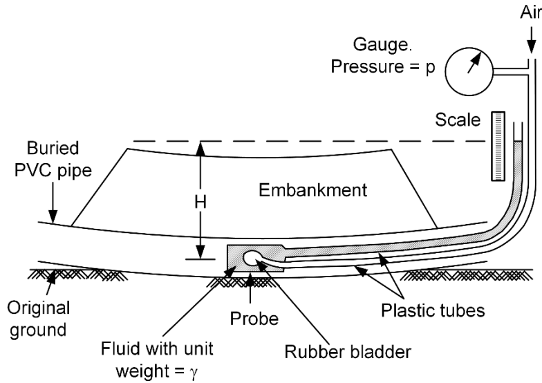
Figure 2-26 Liquid Level System to Continuously Profile Settlements (after Dunnycliff 1993)
