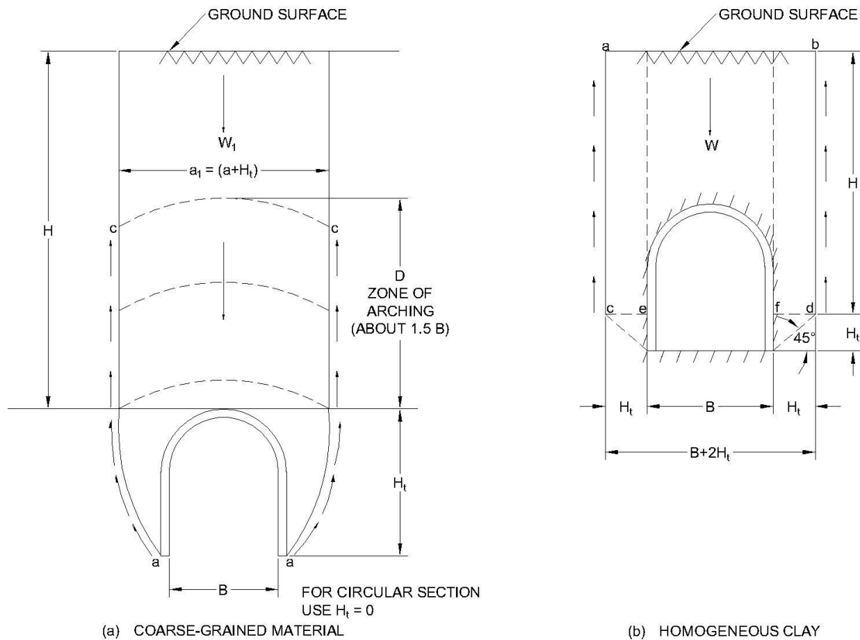
Figure 4-11 Loading Mechanisms for Soft Ground Tunneling
