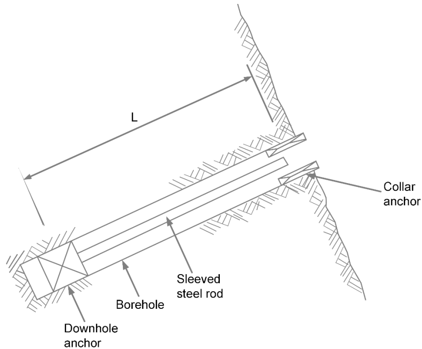
Figure 2-27 Borehole Extensometer (after Dunnycliff 1993)
