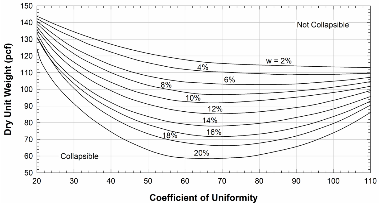
Figure 1-10 Design Charts for Predicting Collapse Behavior of Soils (after Ayadat and Hanna 2007b)
