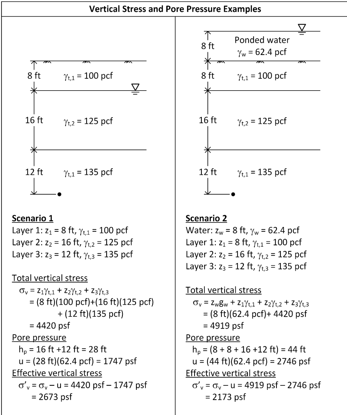
Figure 4-1 Calculation of Vertical Stresses for Hydrostatic Conditions
