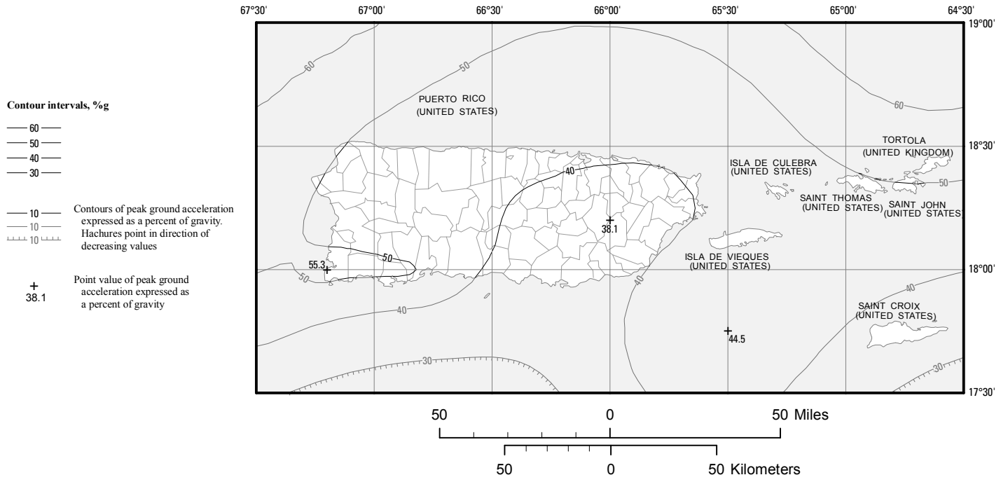
Figure 22-11 MCE geometric mean PGA, %g, Site Class B for Puerto Rico and United States Virgin Islands
